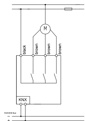
Exemplary circuit diagram AKK-03UP.03 Fancoil
