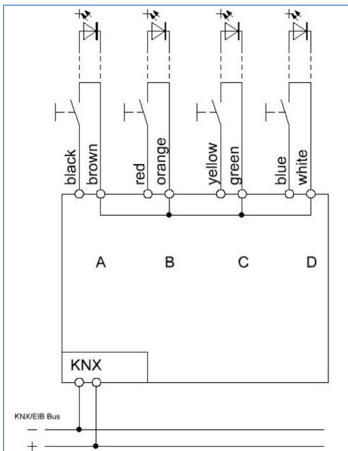
Figure 1: Exemplary circuit diagram BE0400.01- Model with 4 inputs
