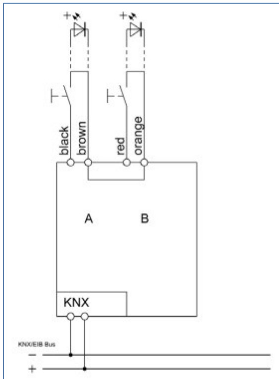
Figure 2: Exemplary circuit diagram BE0200.01- Model with 2 inputs
