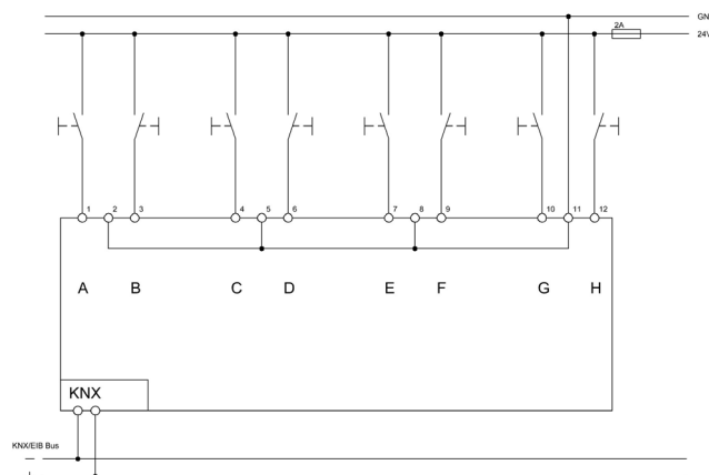
Exemplary circuit diagram BE-08024.01
