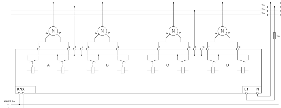
Anschluss JAL-0410.02 - Exemplary circuit diagram JAL-0410.02
