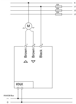
Anschluss JAL-01UP.02 - Exemplary circuit diagram JAL-
