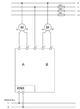
Anschluss JAL-0410.02 - Exemplary circuit diagram JAL-0410.02
