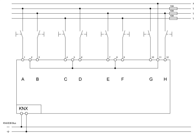
Exemplary circuit diagram BE-08230.02 - Different circuits
